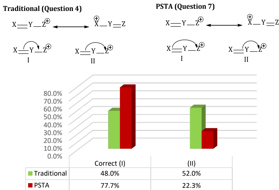
Figure 8. Resonance arrows
